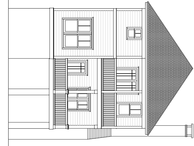
SIDE 2 ELEVATION
